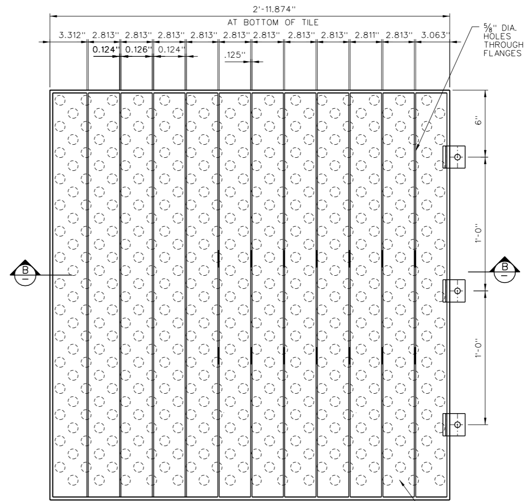
REFLECTED PLAN
