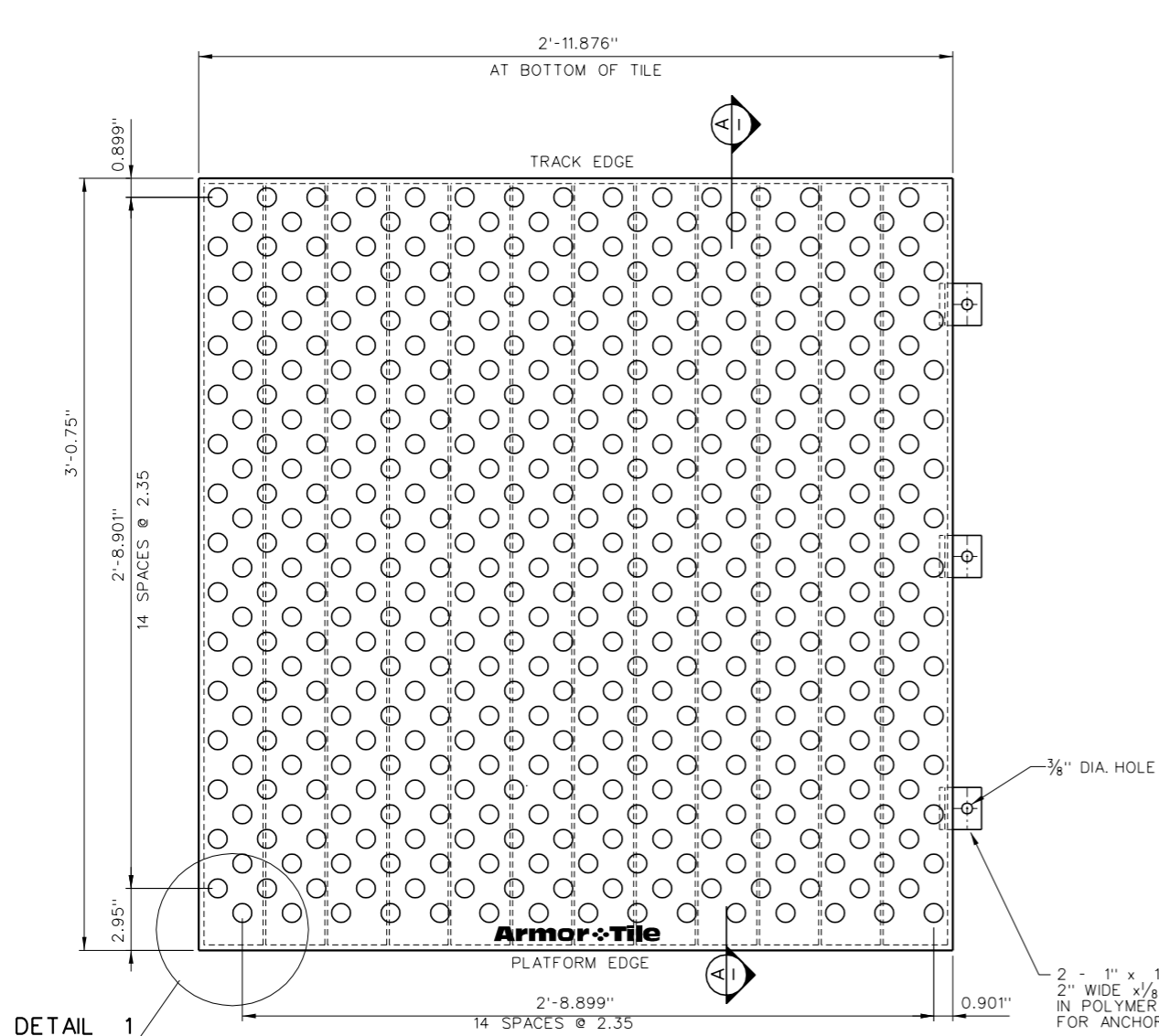
PLAN - TILE
