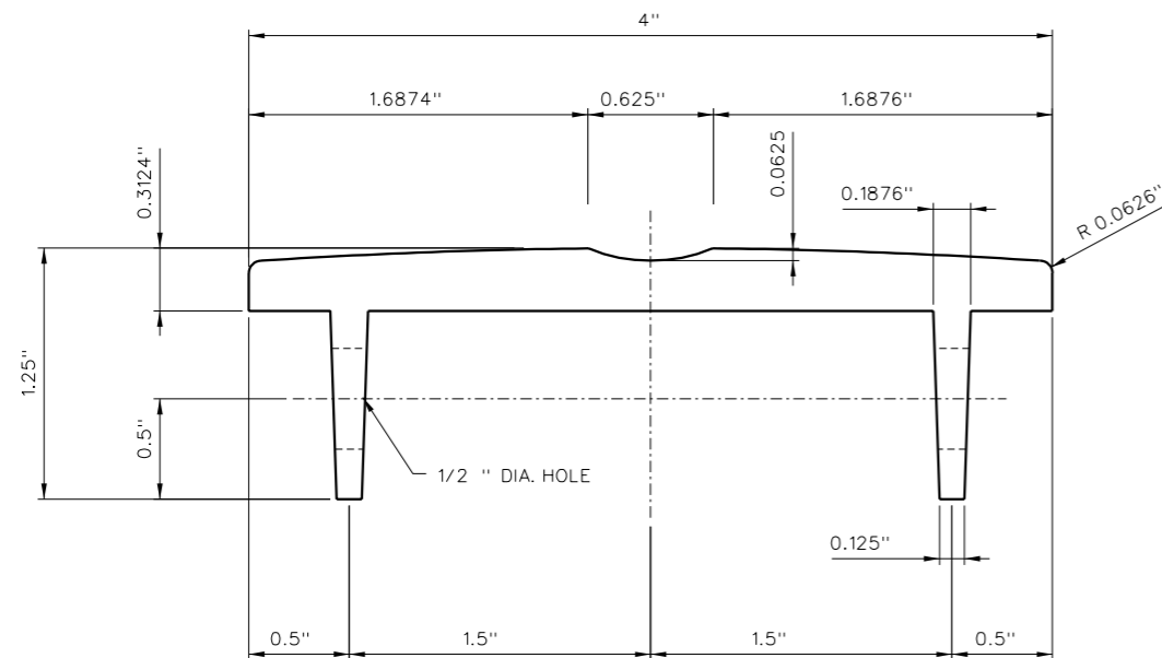
SECTION A-A HALF SCALE
